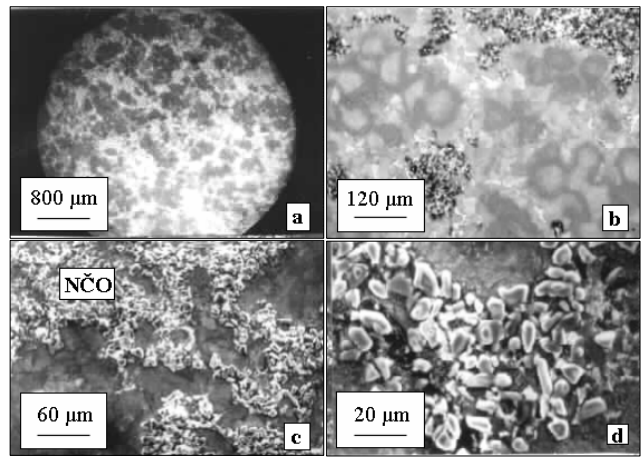
Figure 2: Composites RAR27 + 3 mass % Al_2O_3 , 12\mu m , etched by 6 % nital; a) General structure appearance, b) Appearance of the metal matrix portion, c) Appearance of clusters of the reinforcement particles, d) Detail, one of the clusters
