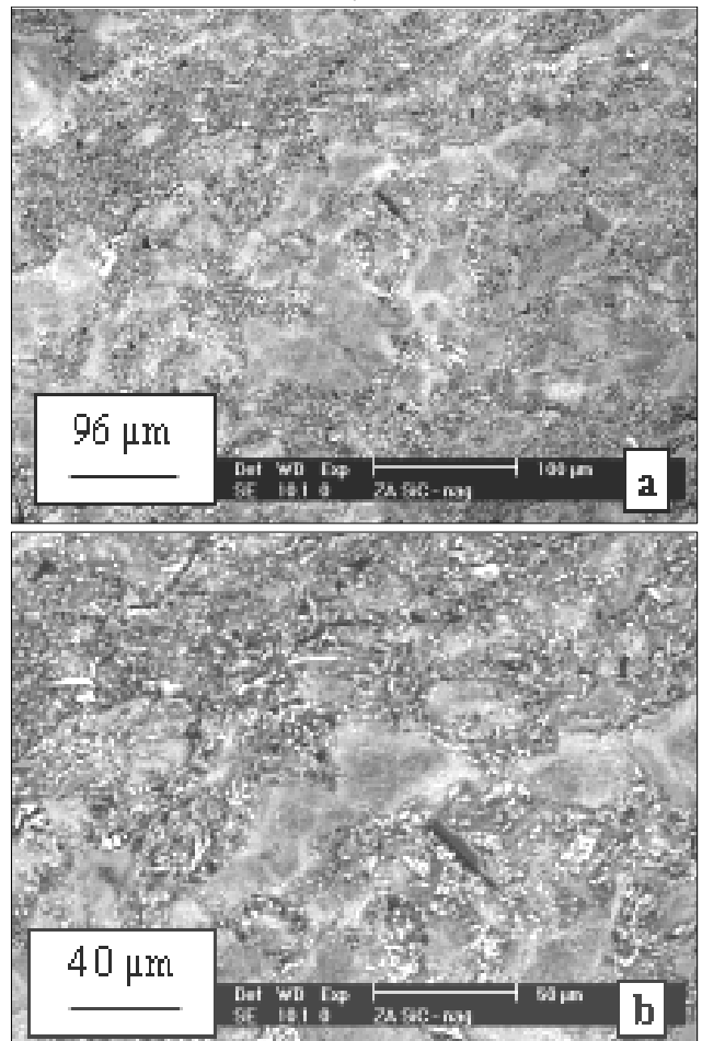
Figure 3: Composite of RAR27 + 3 mass % of SiC , 15\mu m (SEM)
