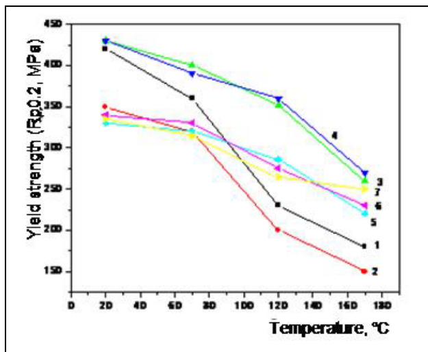
Figure 4: Variation of the yield strength ( R_{p0.2} ) with temperature, for the compression tests [6].
