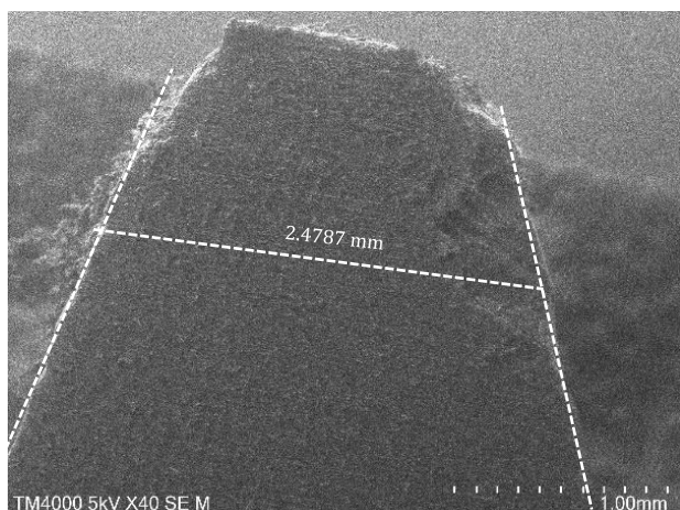
Fig. 16. The thickness of the Onyx material+10%CF tooth is 2.5100 mm.
