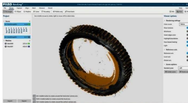
Fig. 6. 3D Scanning of brass worm gear ring.
