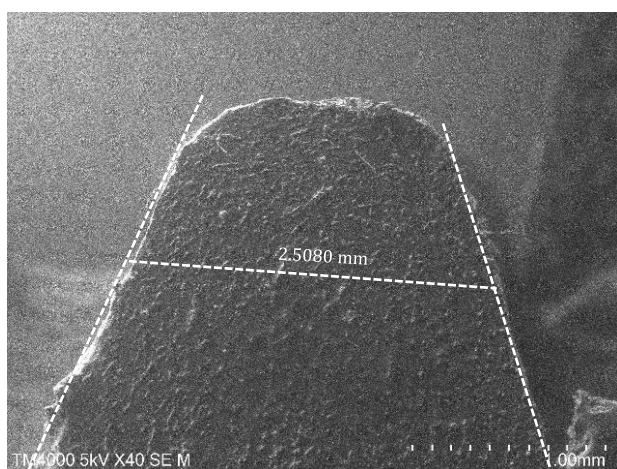
Fig. 17. The comparative tooth thickness without wear is 2.5730 mm.
