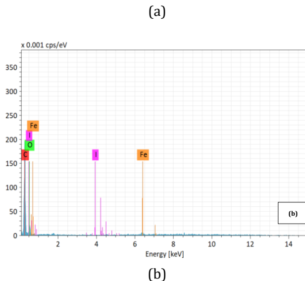
Fig. 3. (a) SEM and (b) EDS material Onyx+10%CF.
