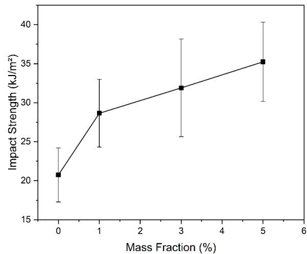
Fig. 6. Impact strength of resin-HA composite.
