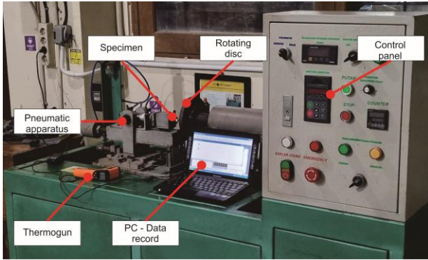
Fig. 2. Tribometry machine.
