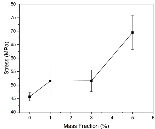
Fig. 3. Tensile Strength of resin-HA Composite.
