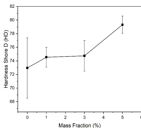
Fig. 7. Hardness Shore D of resin-HA composite.
