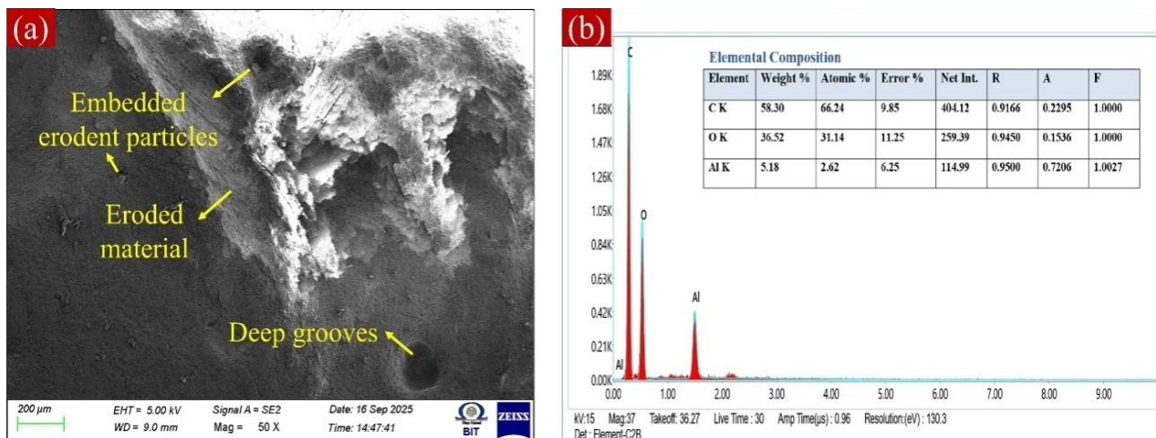
Fig. 18. FESEM of the eroded surfaces with EDS
