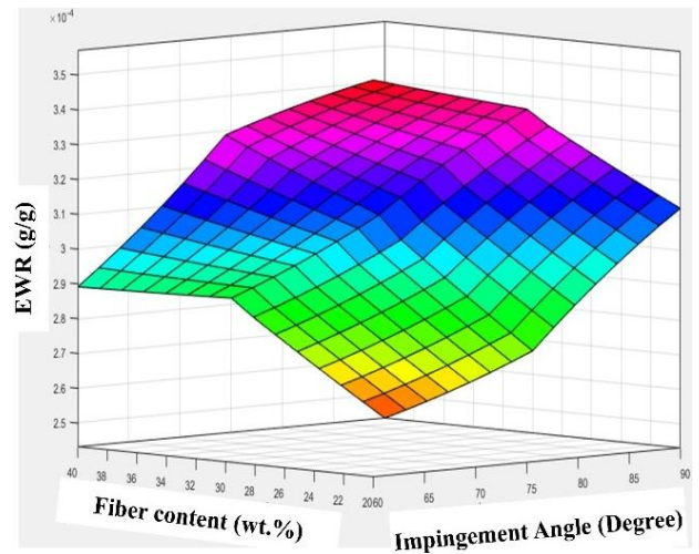
Fig 16c. ANFIS plot for the response erosion wear rate of F-E composites as a function of fiber content and impingement angle.
