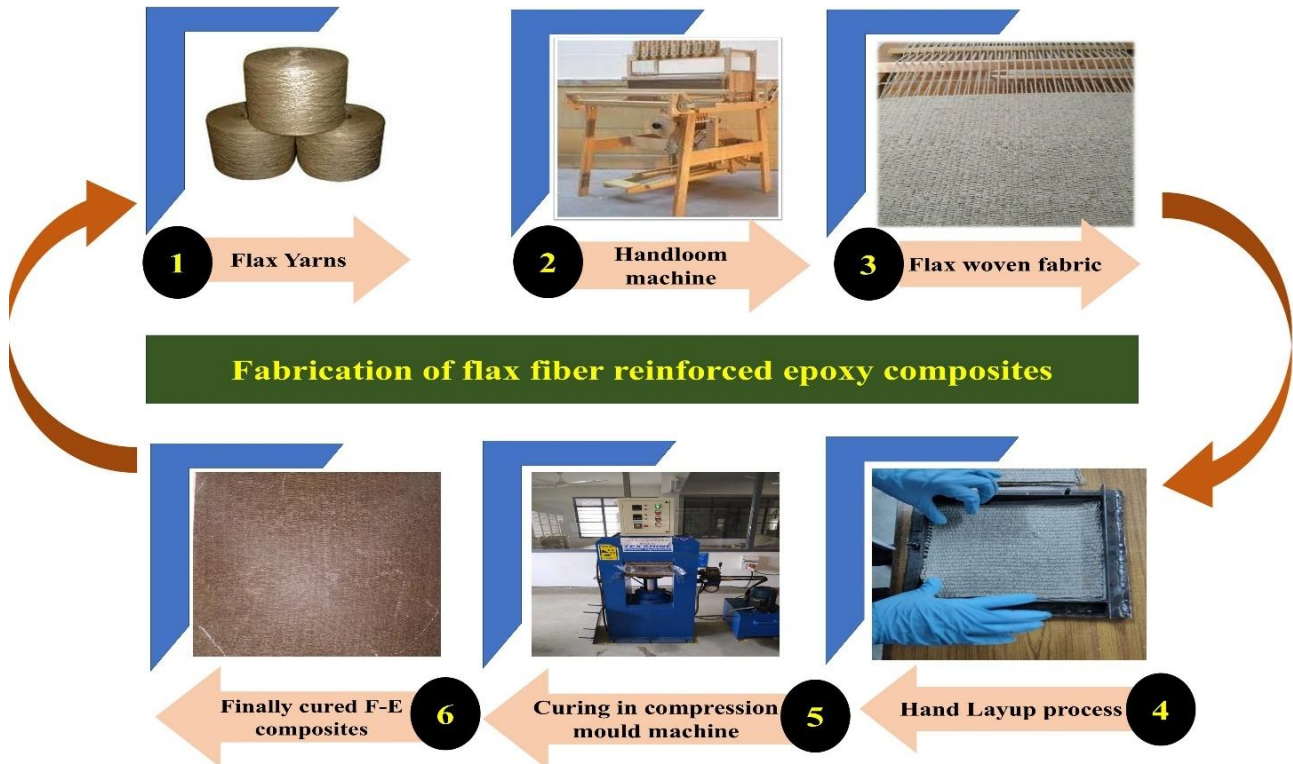
Fig. 2. Steps followed in the preparation of F-E composites.
