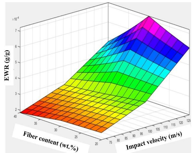
Fig 16b. ANFIS plot for the response erosion wear rate of F-E composites as a function of fiber content and impact velocity.
