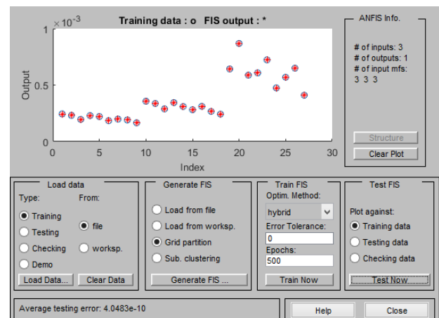
Fig. 8. Validation of input parameter (erosion wear) with Sugeno model in MATLAB (R2017a).
