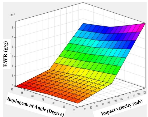
Fig 16a. ANFIS plot for the response erosion wear rate of F-E composites as a function of impingement angle and impact velocity.
