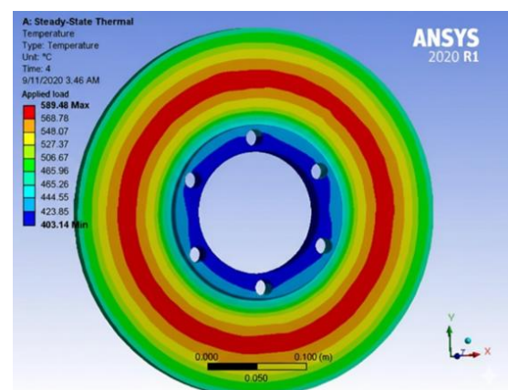
Fig. 3. Brake Disc Thermal Cycling Simulation
