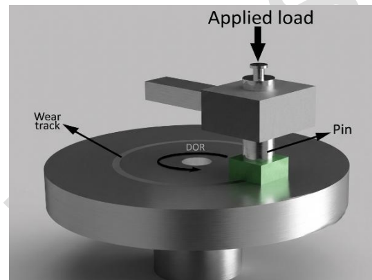
Fig. 2. Pin-on-Disc Wear Test Schematic
