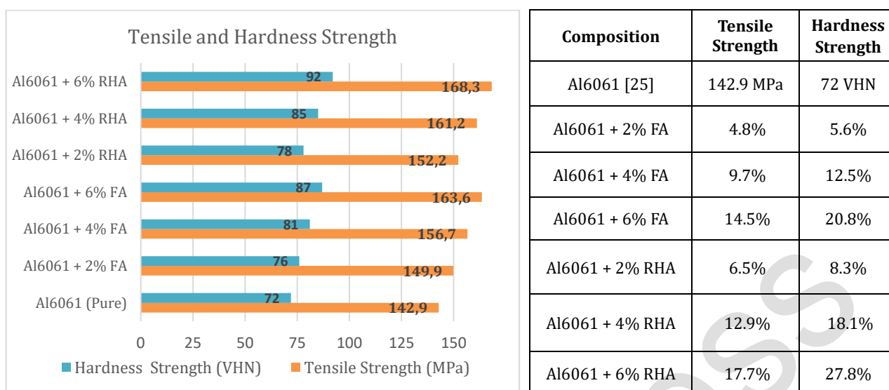
Fig. 11. Tensile and hardness strength (table represents % improvement over base Al6061).
