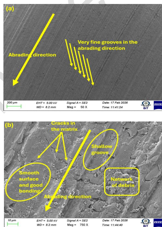
Fig. 17. Worn surface morphology of 0.8 wt% CNF-modified composite (C2): (a) very fine grooves along the abrading direction, (b) smooth surface with shallow grooves, limited matrix cracks, and debris network.
